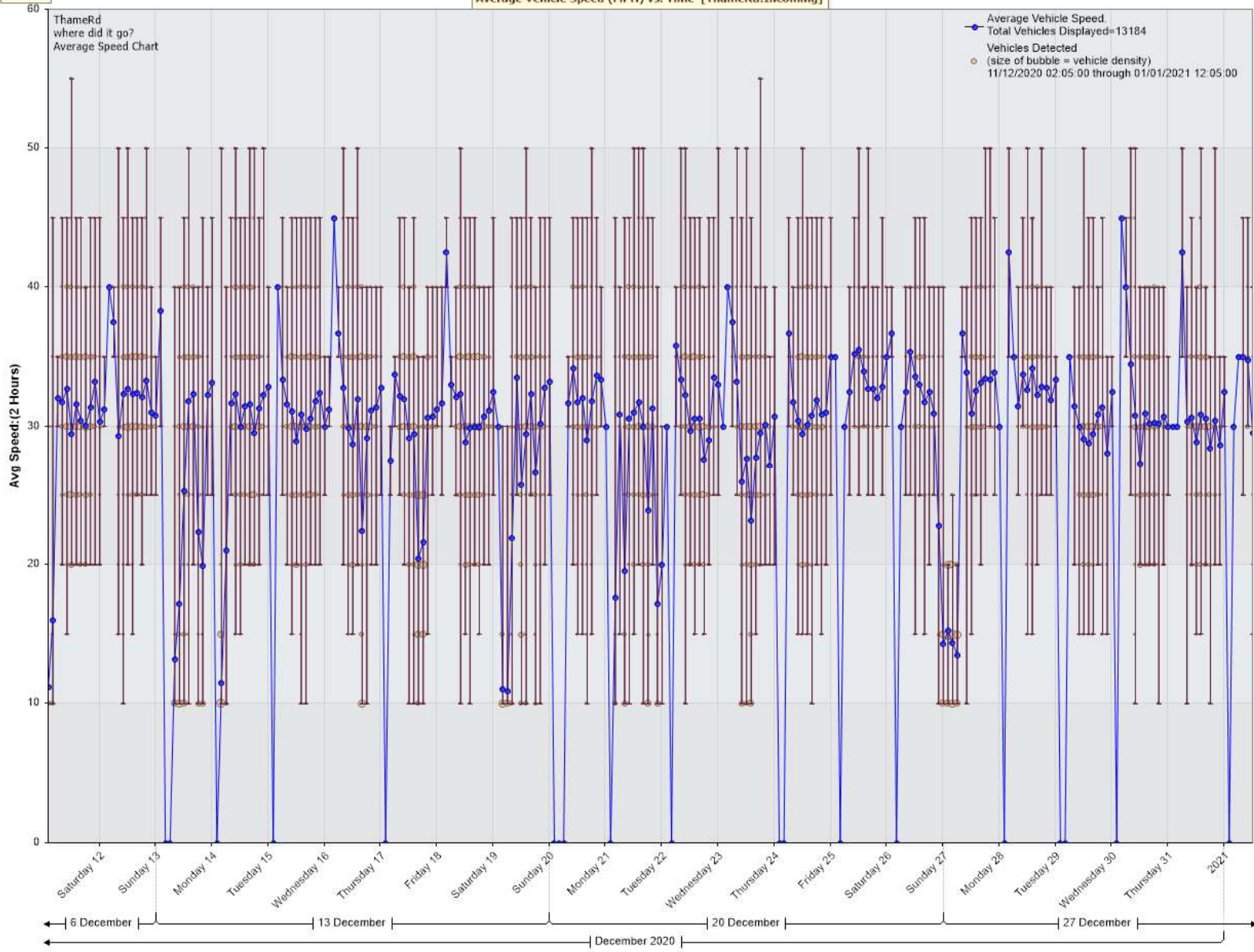
Average Vehicle Speed (MPH) vs. Time [ThameRd:Incoming]
